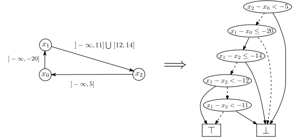
Fig. 8. Compilation of an inconsistent TCSP as a \text{DDD}_\succ representation
