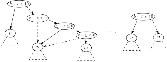
Fig. 5. A non path-feasible DDD (left) and a path-feasible version (right) of this latter
